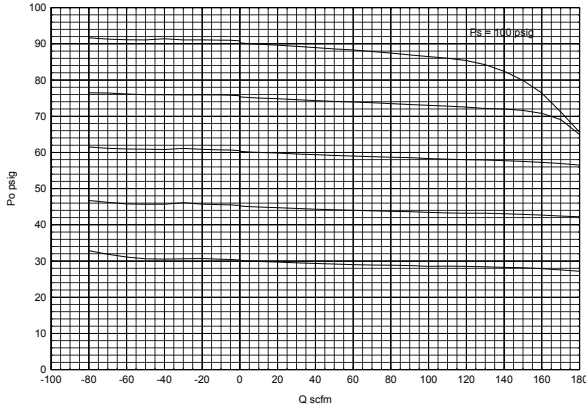
Forward & Exhaust Flow Characteristics Fairchild Model 4514A
