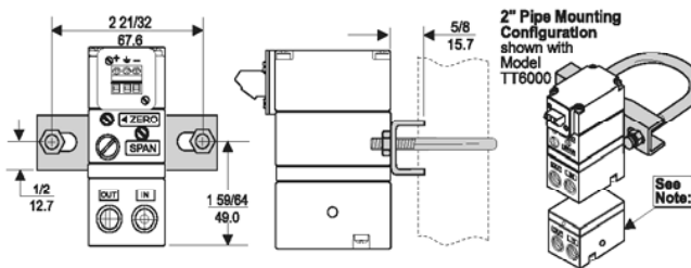
Mounting Bracket: 19254-1
