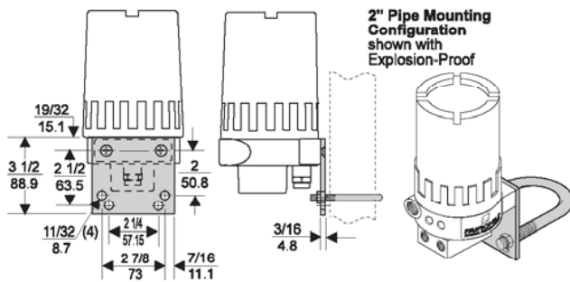
Mounting Bracket: 18187-1
