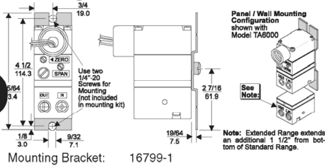
Mounting Bracket: 16799-1
