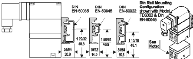
Mounting Bracket: 16893-1
